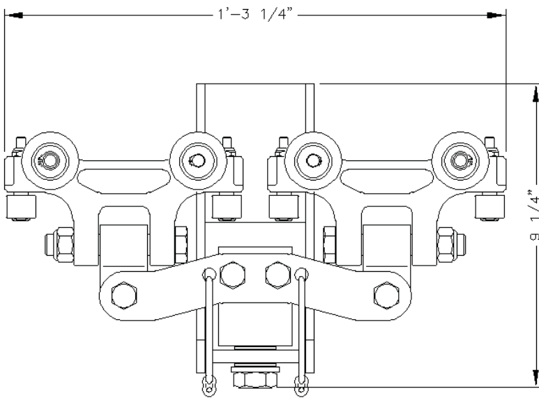
22600 ETA-4/5 ARTICULATING LOW HEAD ROOM END TRUCK DUAL TROLLEY END TRUCK AT EACH END OF CRANE GIRDER. RATED LOAD: 1000 lbs. WEIGHT: 16 lbs.
