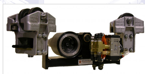
I-beam (can run on curved rail)
