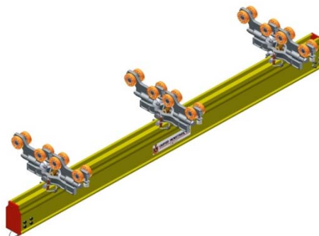
Tri-Bridge with Dual End Trucks
