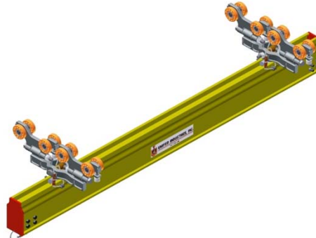
Tri-Bridge with Dual End Trucks
