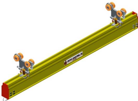
Single Girder Bridge with Low Headroom End Trucks
